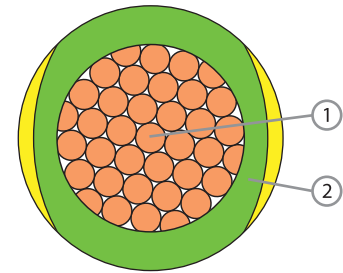
Component 1. Plain Annealed Copper Wire 2. PV Compound
