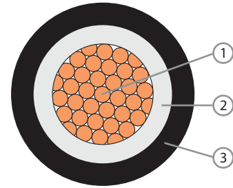
Component 1. Plain Annealed Copper Wire 2. Cross-linked Polyethylene Compound 3. PVC Compound
