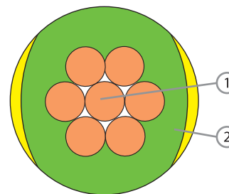
Component 1. Plain Annealed Copper Wire 2. PV Compound
